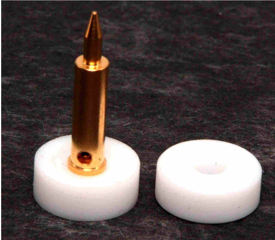
2 identische PTFE-Scheiben, die vertauschbar sind. 2 identical PTFE-discs which can be changed.
